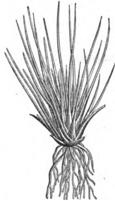
FIG. 360. — Isoetes lacustris ; \times \frac{1}{2} . (From Kerner.)
